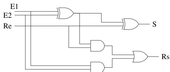
FIGURE 3 – Circuit logique
